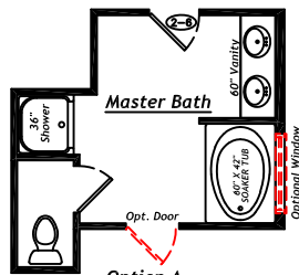
Option A 60"x42" Soaker Tub w/ 36" Shower Dual Vanity W/ Double Sink Enclosed Toilet
